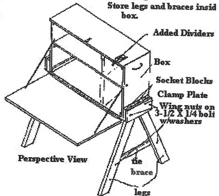
View of Socket Blocks in place on Box End
